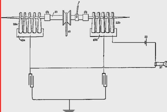
FIG 3.—ARRANGEMENT OF RECEIVING APPARATUS. MURGAS SYSTEM OF WIRELESS TELEGRAPHY.
