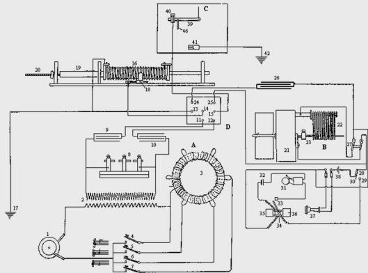
FIG 1.—APPARATUS AND CONNECTION AT ONE STATION—MURGAS SYSTEM OF WIRELESS TELEGRAPHY.
